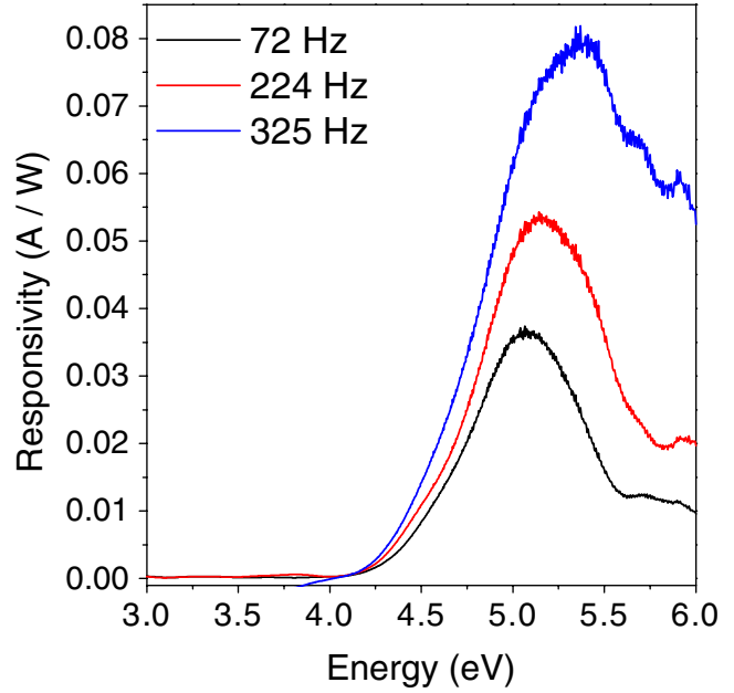
Figure 4. Responsivity spectra for a typical undoped single \text{Ga}_2\text{O}_3 nanowire obtained at different chopper frequencies. The bias voltage was 500 V.
