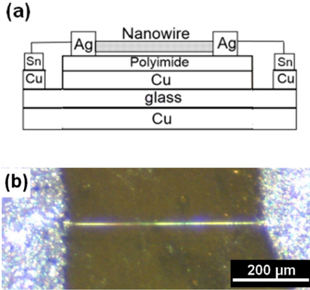
Figure 2. (a) Scheme of the sample holder used for PC measurements. (b) Optical image of one of the prepared \text{Ga}_2\text{O}_3 nanowires tested as a photodetector.
