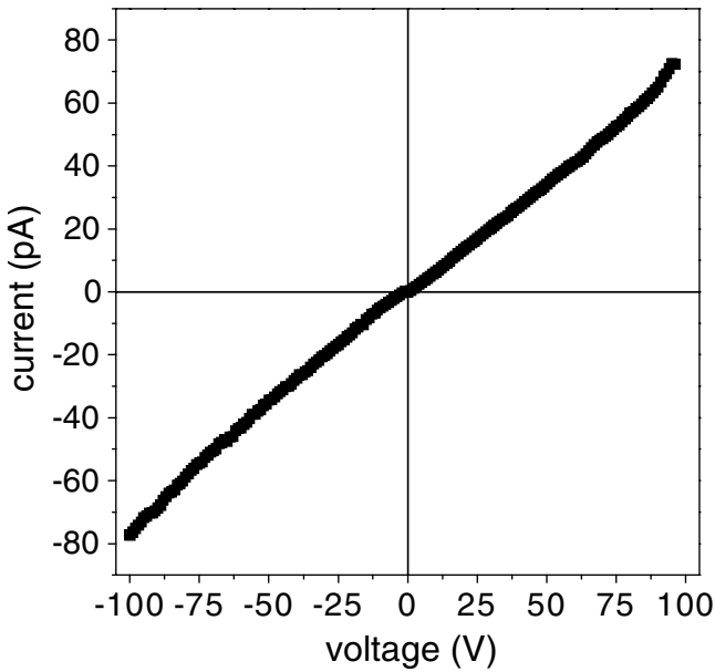
Figure 3. I – V characteristic of a single undoped \text{Ga}_2\text{O}_3 nanowire obtained in dark and air conditions.
